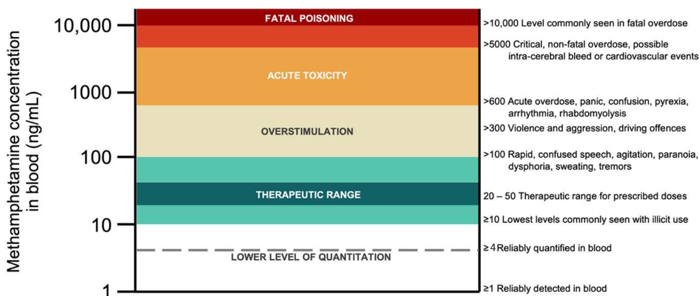
Figure 5: Methylamphetamine concentrations in blood and associated health effects
