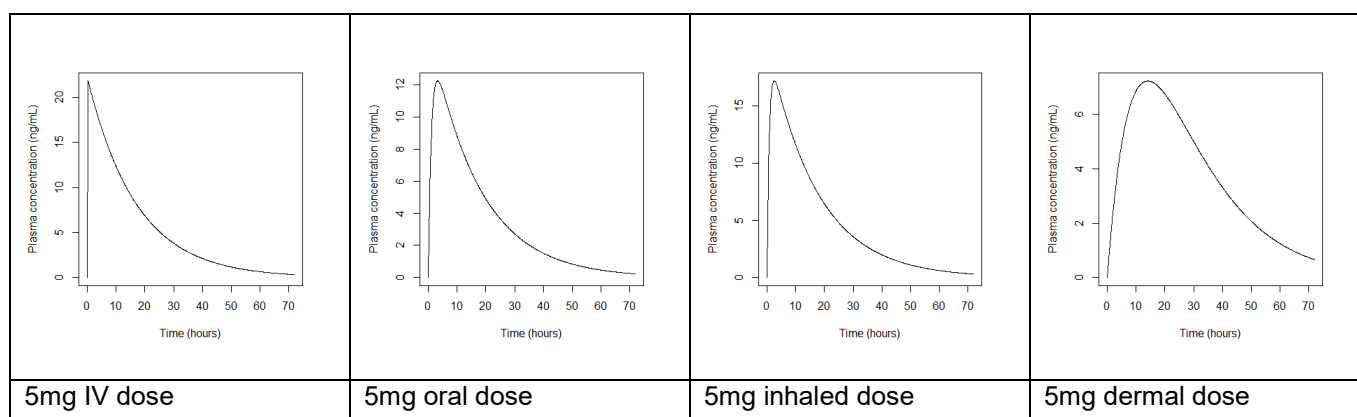
Figure 3: Pharmacokinetic profiles of single 5mg intravenous (IV), oral, inhaled and dermal doses of methylamphetamine in adults
